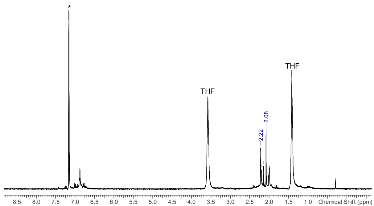
^1\text{H} -NMR-Spektrum in \text{C}_6\text{D}_6
