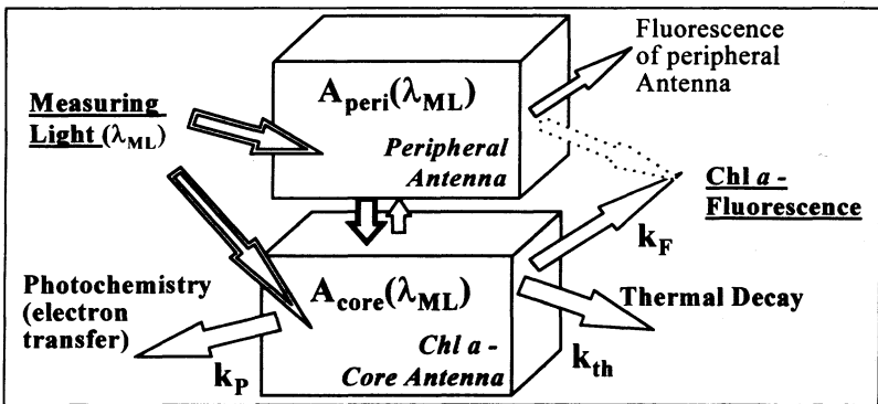
Fig. 3 Creation and decay of excited states in the PS II. An excited state is created by absorption of a photon; A_{\text{peri}}(\lambda_{\text{ML}}) and A_{\text{core}}(\lambda_{\text{ML}}) are the absorption coefficients (precisely spoken: the absorption cross-section at \lambda_{\text{ML}} ) of the peripheral and the core antenna, respectively. Due to rapid hopping between antenna pigments a so-called 'exciton equilibrium' is established. Then the excited state decays via four major pathways: (1) initiation of charge separation (electron transfer), (2) thermal dissipation (non-radiative decay), (3) emission of a fluorescence photon (radiative decay), (4) formation of triplet states (intersystem crossing). Triplet-formation is of particular relevance with respect to initiation of photodamage, but due to its extremely low yield this decay process is, in the present context, negligible. Due to REE occurrence the rate constants for excited state decay ( k_p , k_{\text{th}} , k_F ) are independent of the excitation wavelength (i.e. \lambda_{\text{ML}} , the wavelength of the measuring light). In case the primary quinone acceptor is singly reduced ( F_M -state), photochemistry is inhibited ( k_p = 0 ) and the fluorescence yield is maximal. For non-reduced Q_A ( F_0 -state), the fluorescence yield is minimal.
