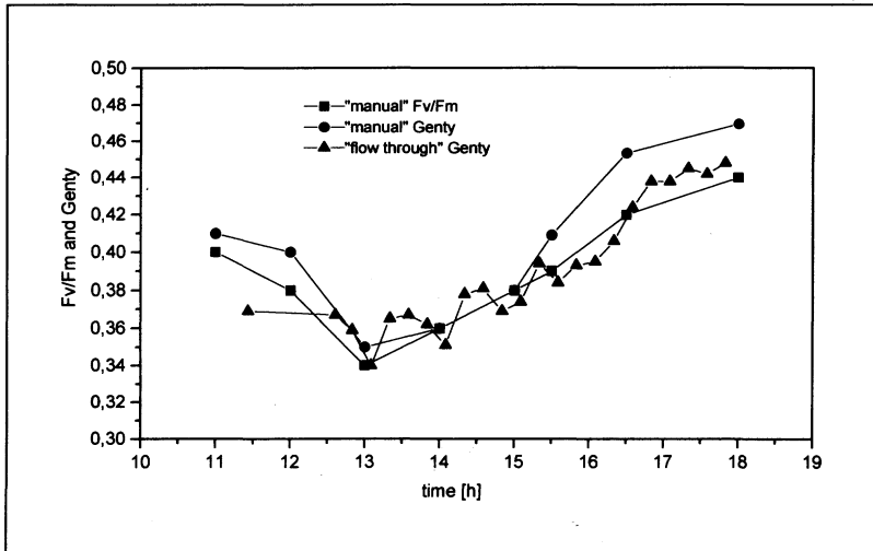
Fig. 2 Maximum and operational quantum yields versus daytime
