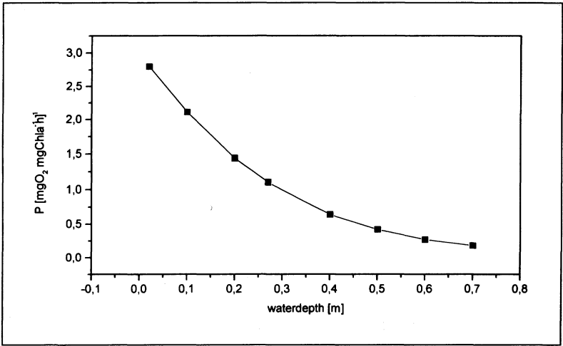
Fig. 6 Calculated photosynthetic rate [ mgO_2\ mgChla^{-1}\ h^{-1} ] versus depth [m].
