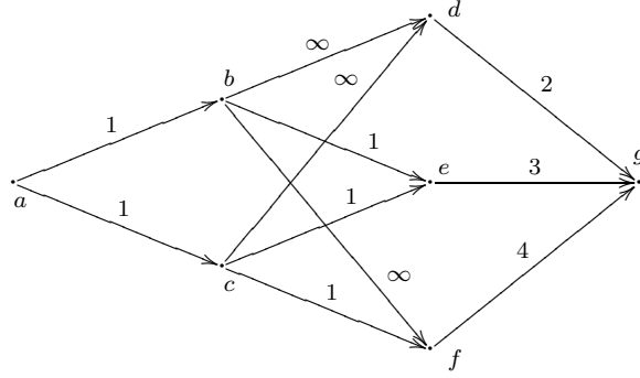
Figure 1: The digraph for the vector \mathbf{a} .
